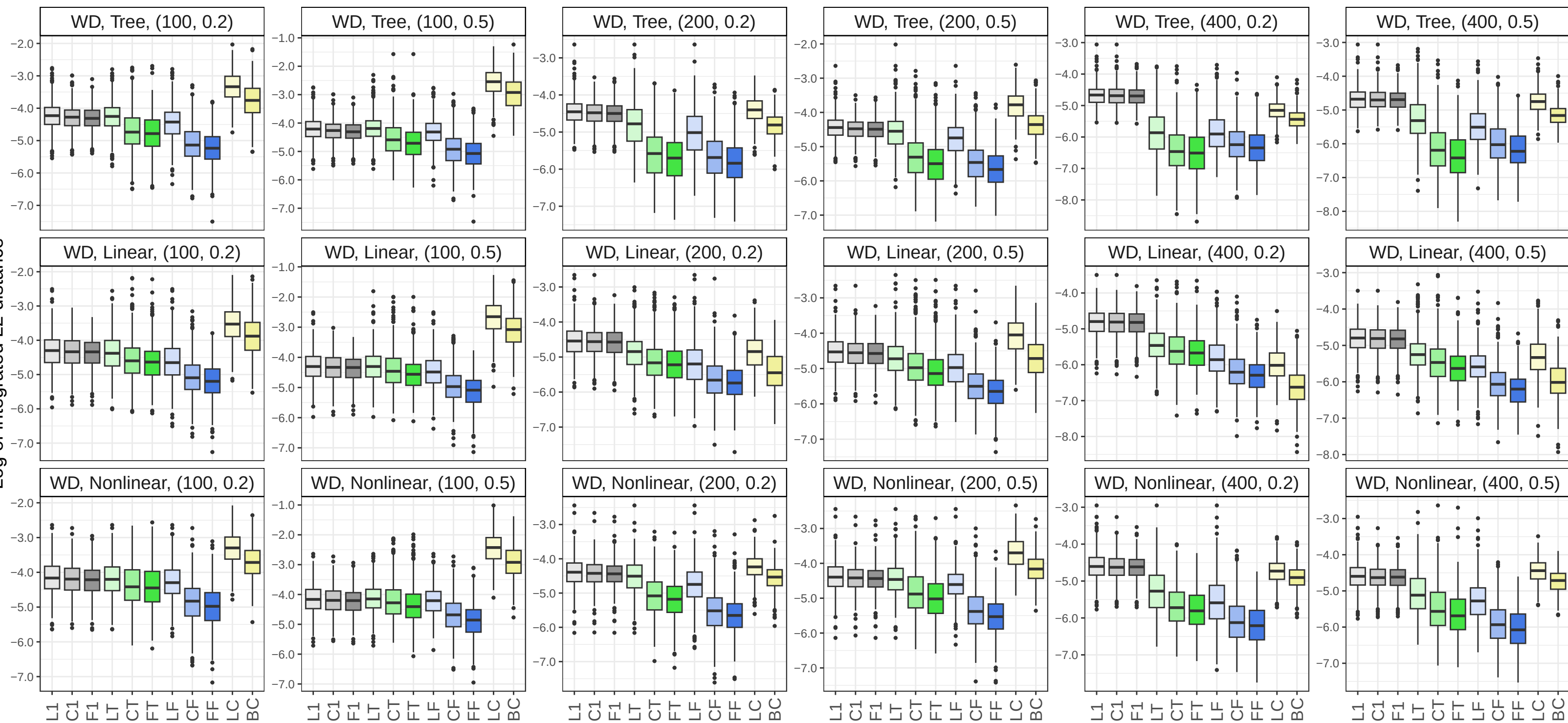
Method
