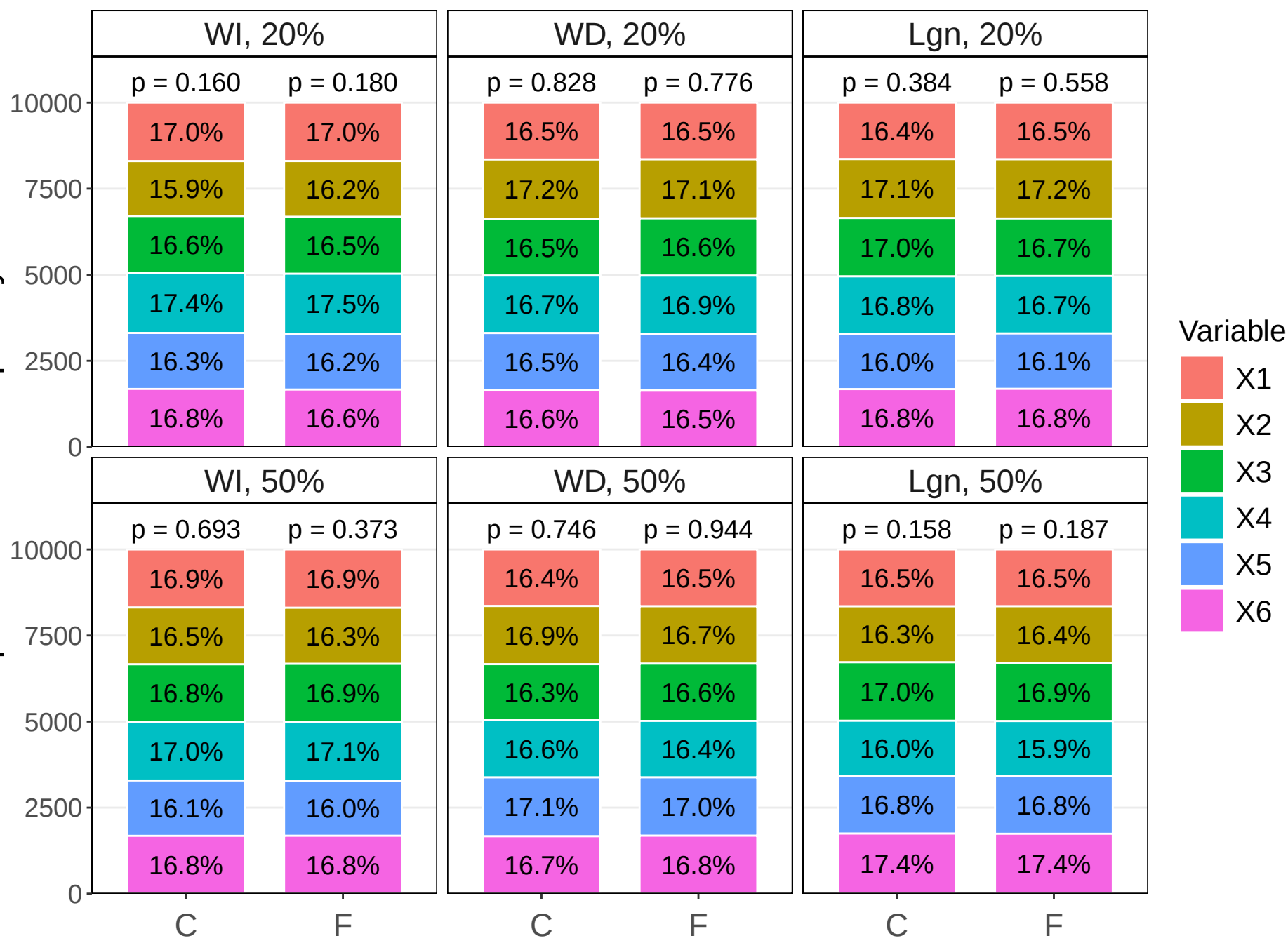
Split-selection frequency
