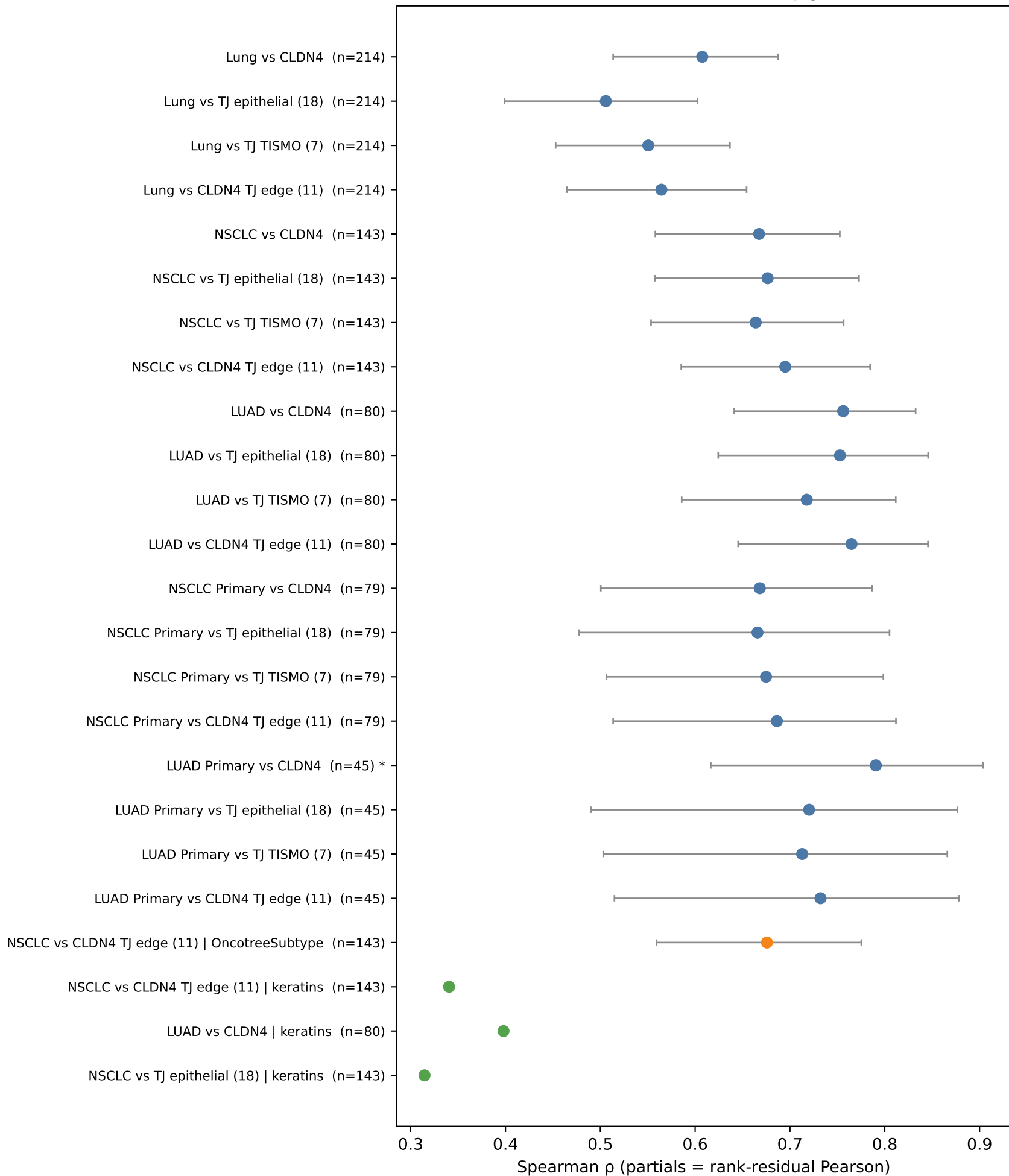
Part1 RNA: TACSTD2 vs locked TJ gene scores
