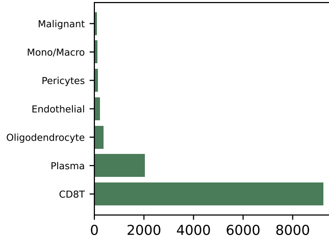
GSE143423 12,193 cells
