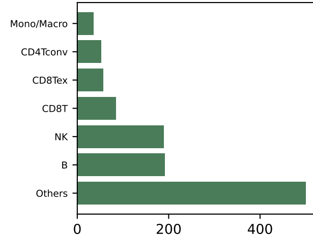
GSE127471 1,108 cells
