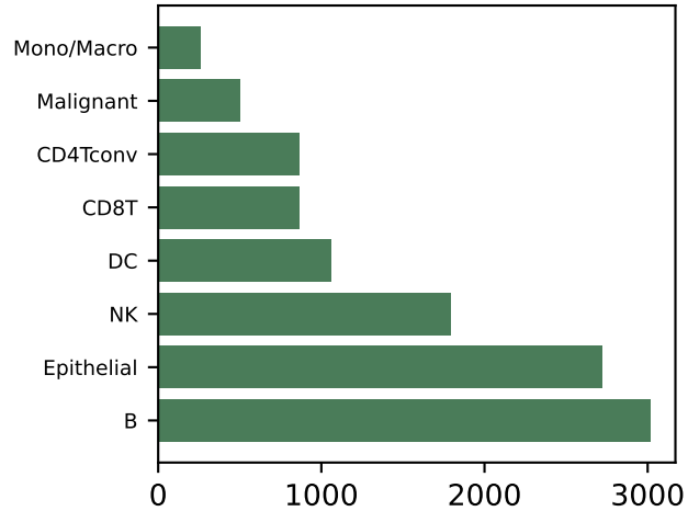
GSE149655 9,591 cells
