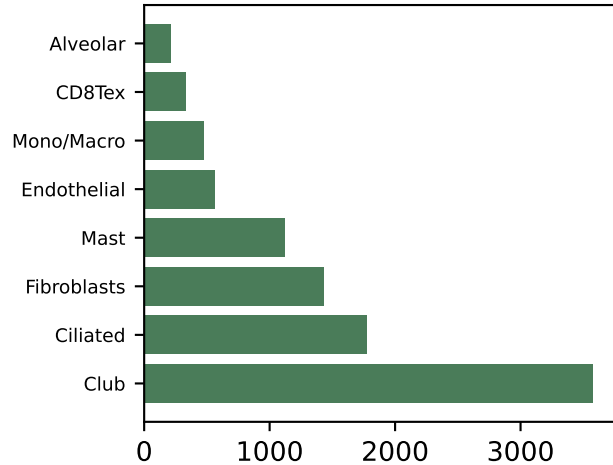
GSE149655 9,591 cells
