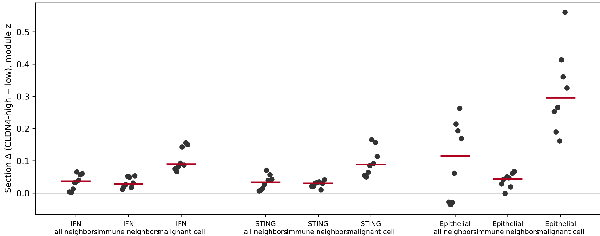
50 \mu\text{m} neighborhood scores (intrinsic has no radius)
