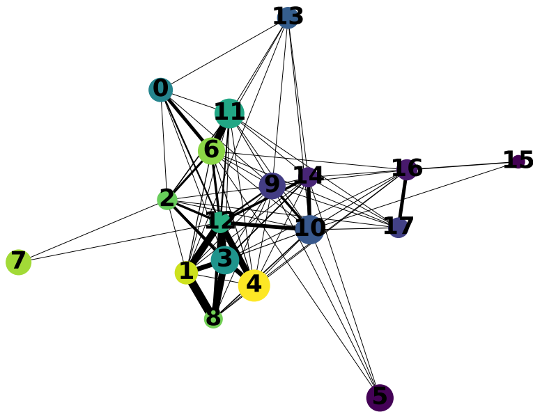
PAGA (Leiden) colored by mean CLDN4
