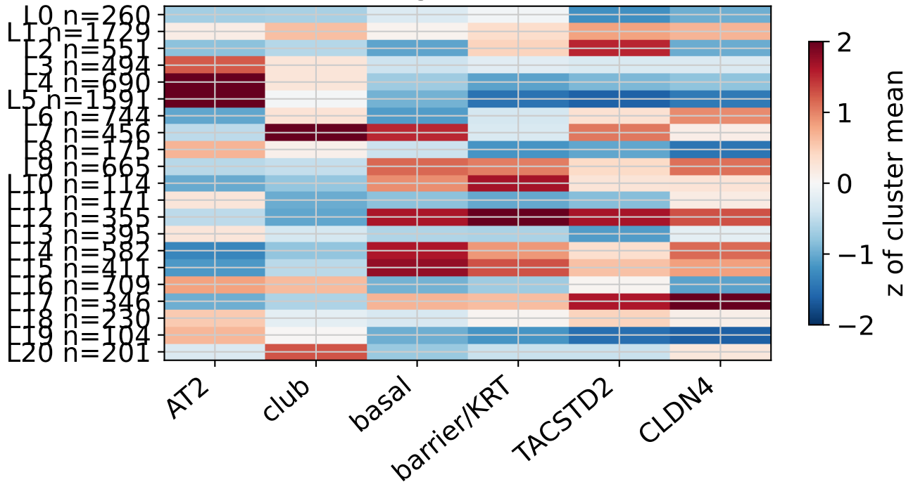
Leiden vertices: lineage scores vs TACSTD2/CLDN4
