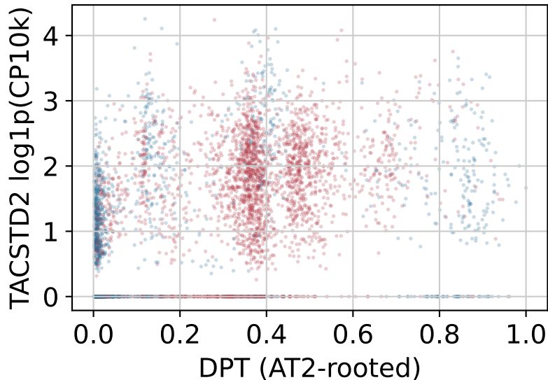
TACSTD2 vs DPT cell-level \rho=0.39 (descriptive)
