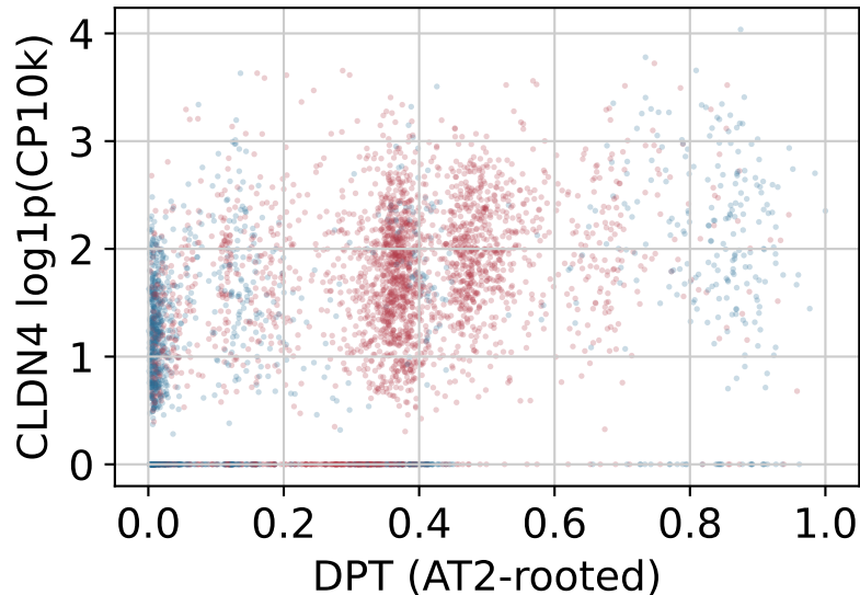
CLDN4 vs DPT cell-level \rho=0.41 (descriptive)
