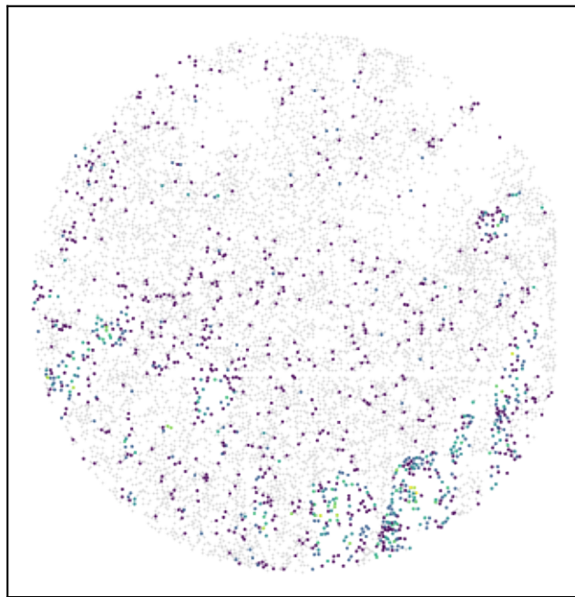
Lung12 tumor log 1 p(CLDN4)
