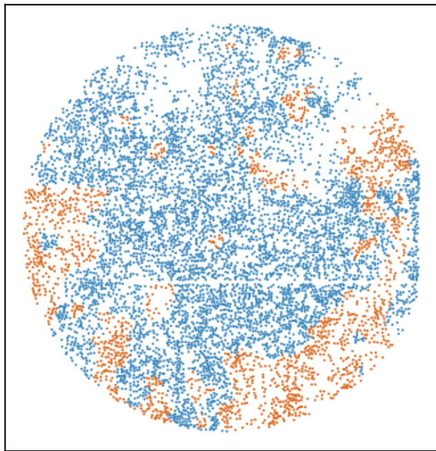
Lung12: CLDN4-high (orange) vs low (blue)
