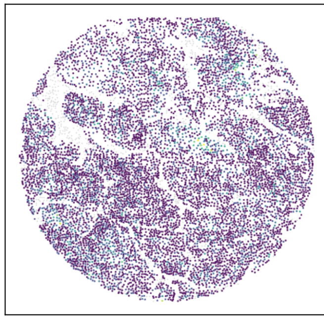
Lung6 tumor log 1 p(CLDN4)
