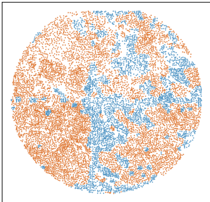
Lung6: CLDN4-high (orange) vs low (blue)
