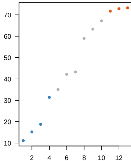
GSE123902
