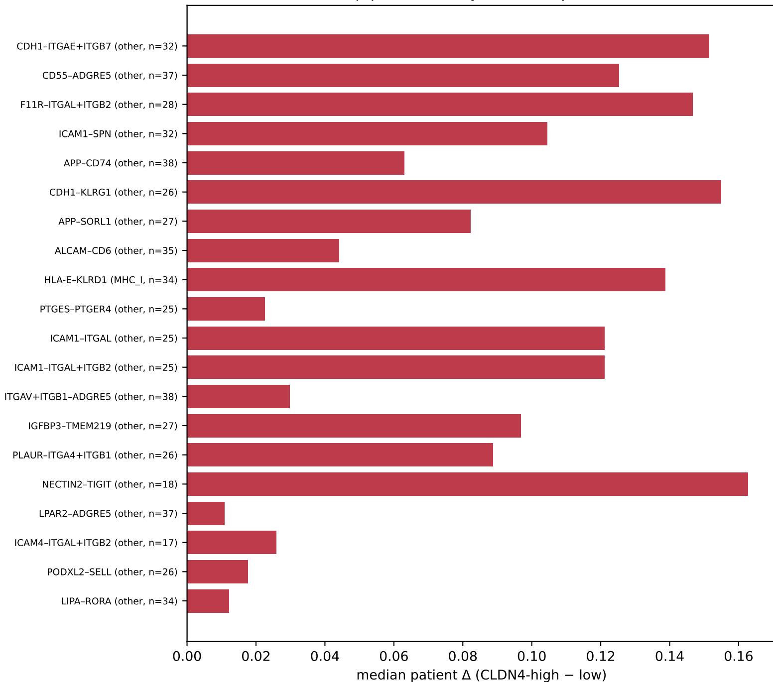
Top paired hits by Wilcoxon p n=40
