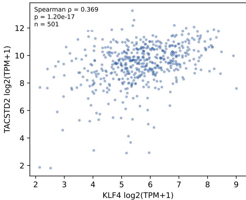
TCGA-LUSC KLF4 vs TACSTD2
