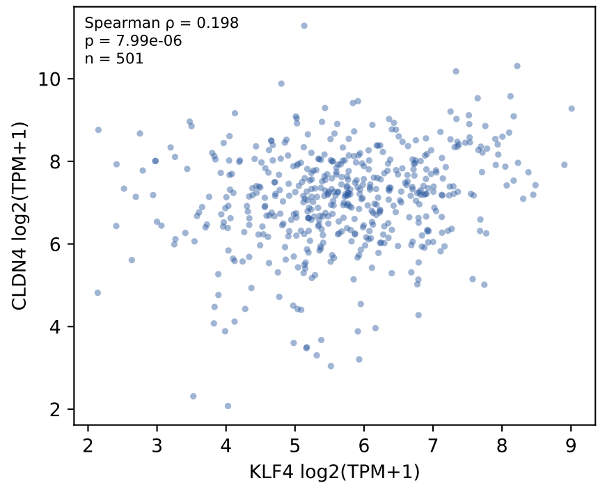
TCGA-LUSC KLF4 vs CLDN4
