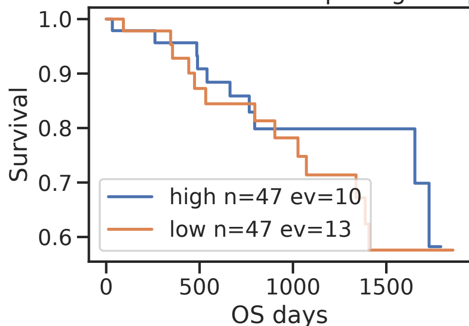
LSCC TACSTD2 OS median-split logrank p=0.2908
