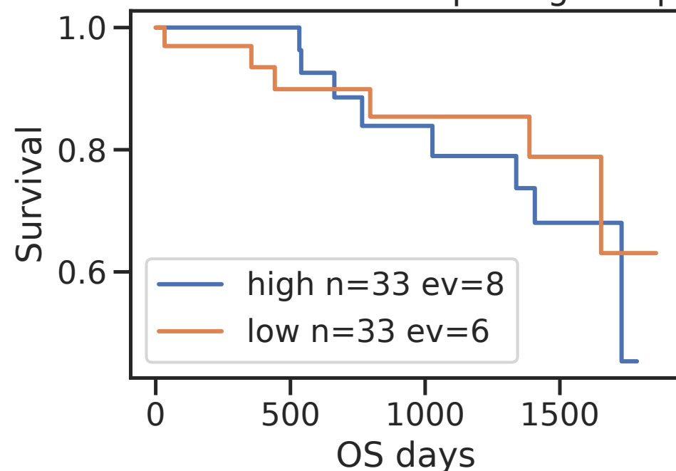
LSCC CLDN4 OS median-split logrank p=0.0008
