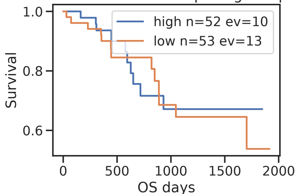
LUAD TACSTD2 OS median-split logrank p=0.1708
