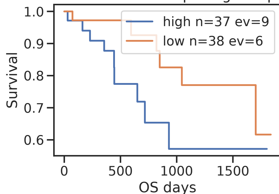
LUAD CLDN4 OS median-split logrank p=0.0008
