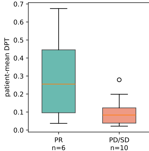
n=16 (PR 6 vs PD/SD 10), \Delta\text{med}=+0.172 , r=+0.0
