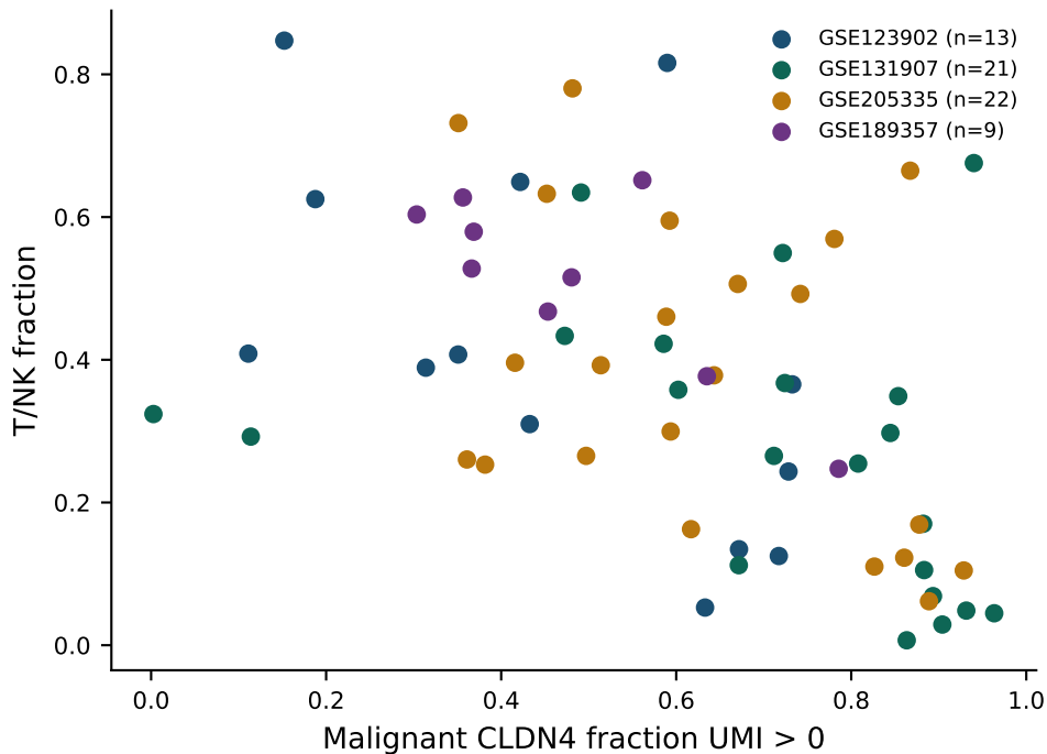
Locked CLDN4 %pos vs T/NK DL \rho = -0.531
