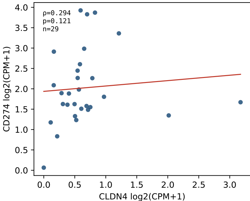
GSE121810 CLDN4 vs CD274
