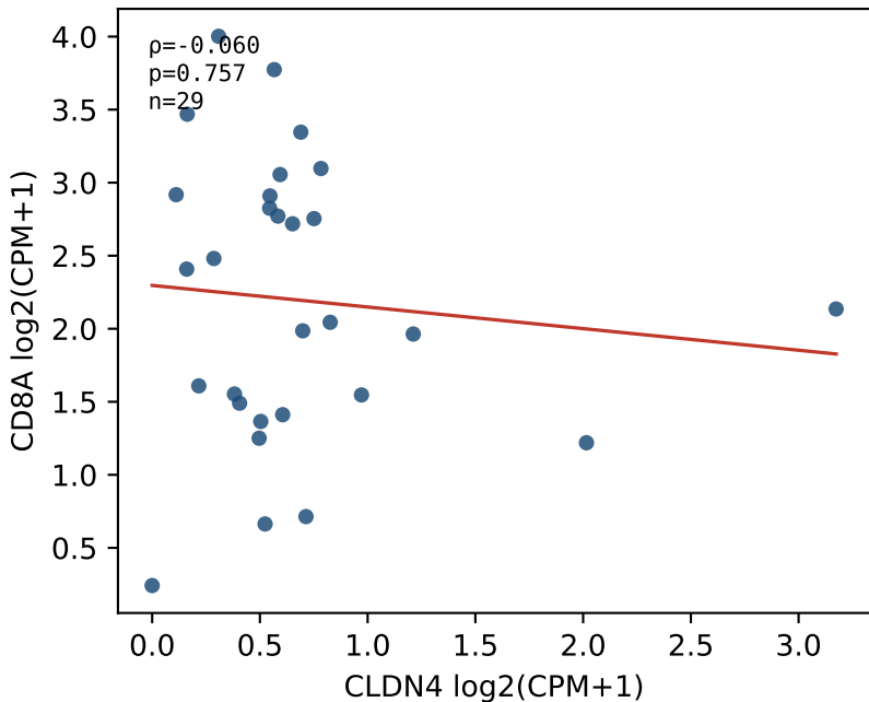
GSE121810 CLDN4 vs CD8A
