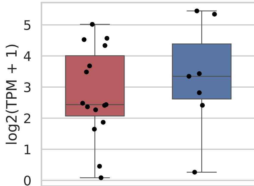
TACSTD2
