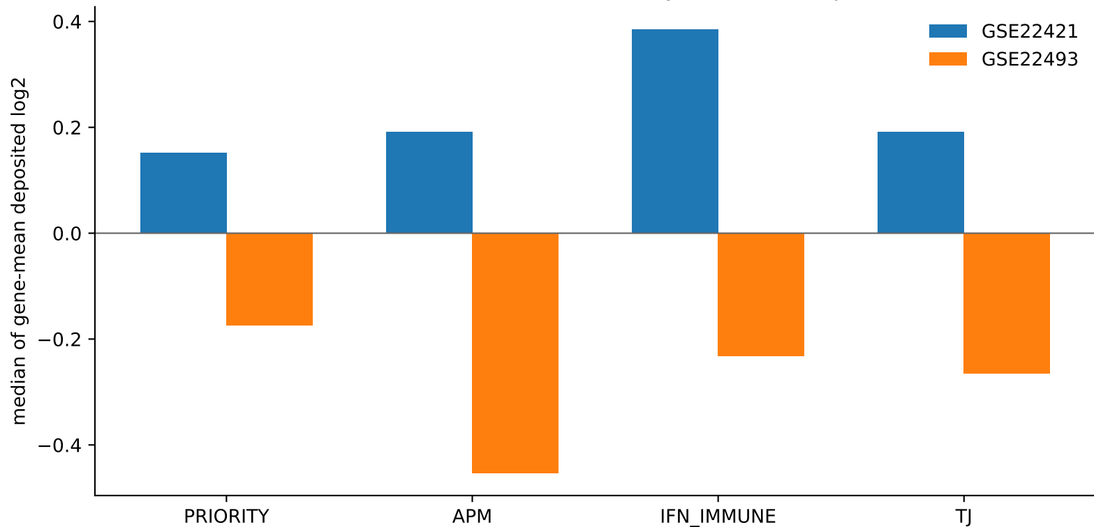
Gene-set location vs 0 (n=3 arrays each; descriptive)
