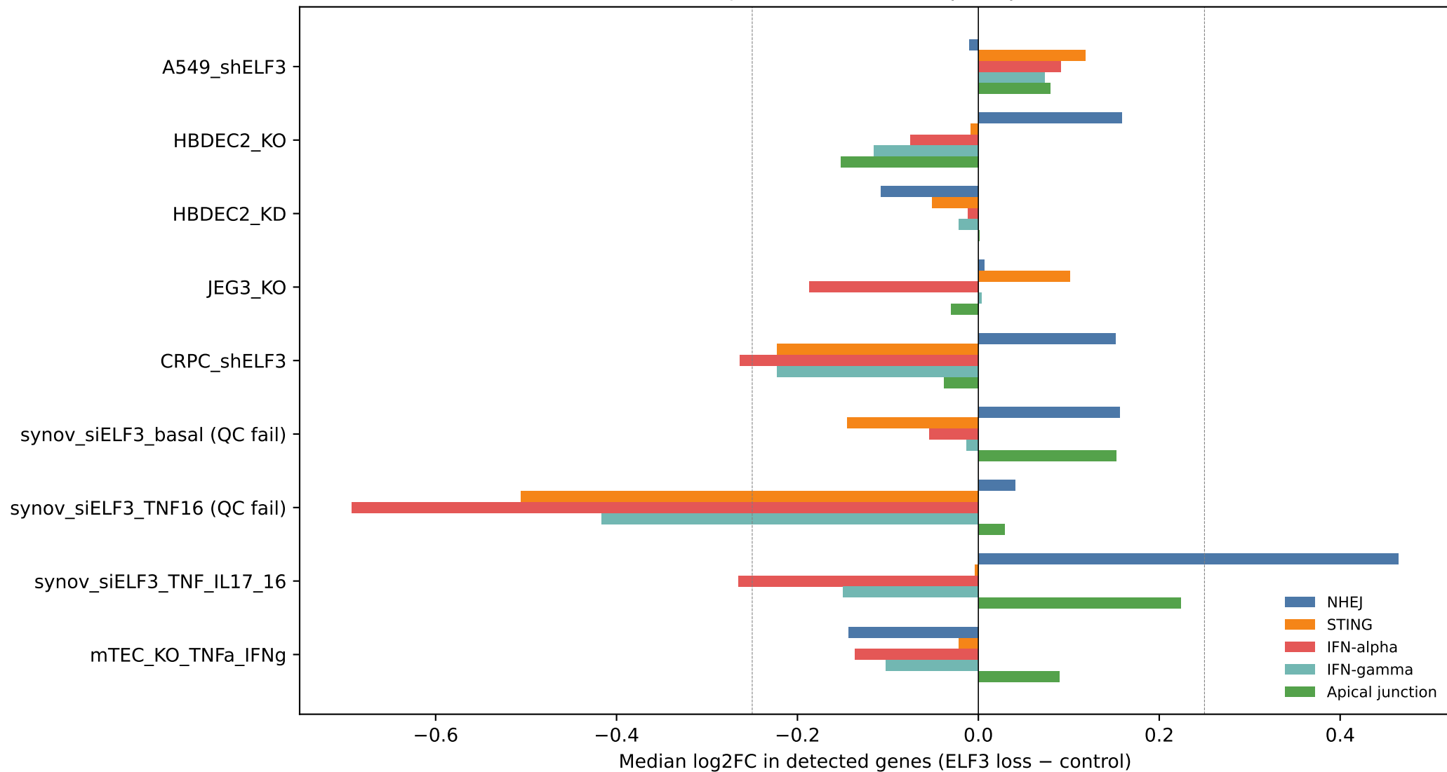
ELF3 loss: NHEJ, STING, IFN, and apical-junction control
