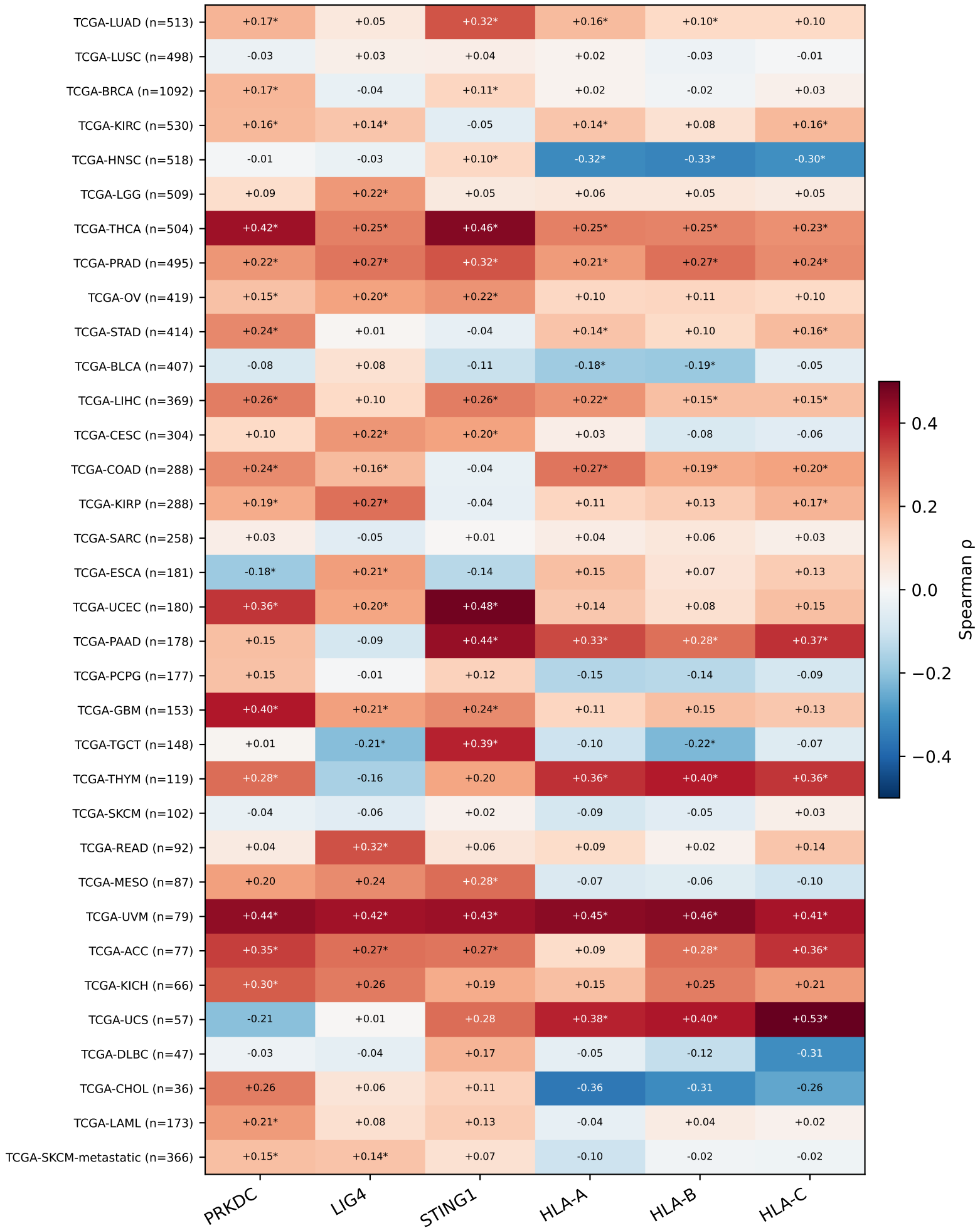
TCGA CLDN4 Spearman \rho (Toil). LUAD/LUSC at top; LAML blood and SKCM metastatic at bottom * exploratory/family q < 0.05 ; color scale \pm 0.5
