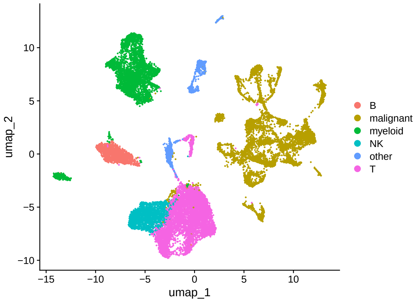
Harmony UMAP by cell class
