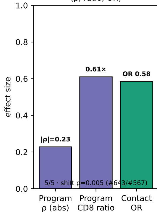
C. CLDN4/TJ program cold (p, ratio, OR)
