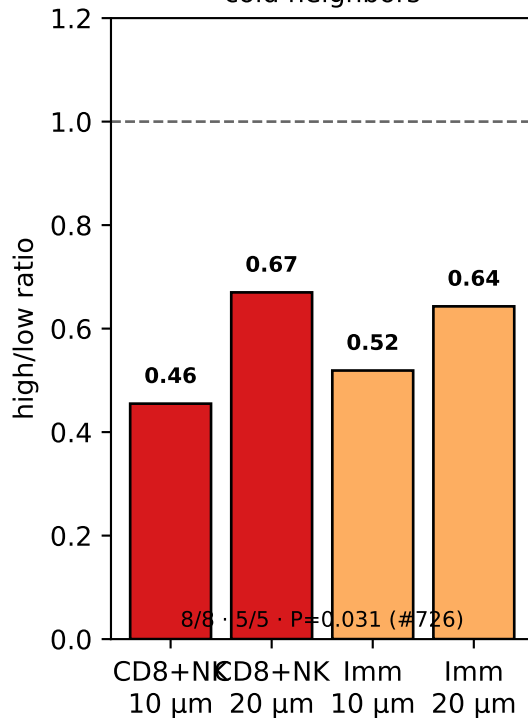
B. TACSTD2-high cold neighbors
