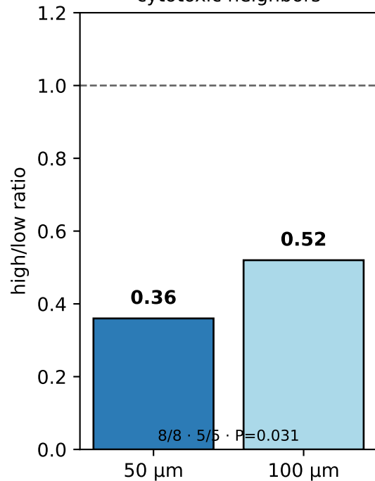
A. LOCKED CLDN4 cytotoxic neighbors
