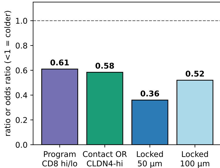
CLDN4 / program cold metrics (CosMx He2022)
