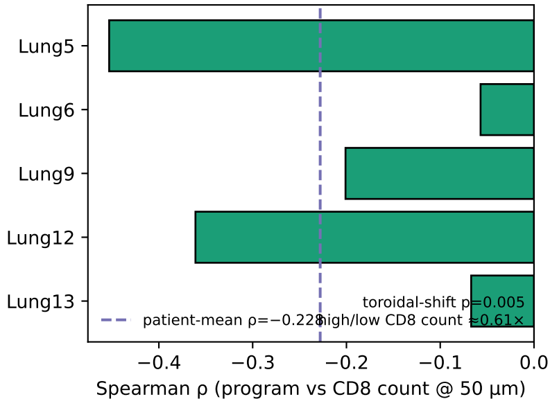
CLDN4 epithelial program cold (PR #643; 5/5 patients)
