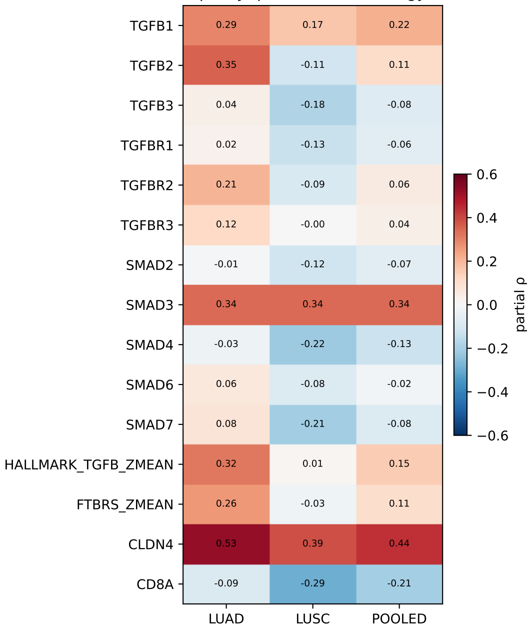
Partial Spearman vs TACSTD2 (purity; pooled also histology)
