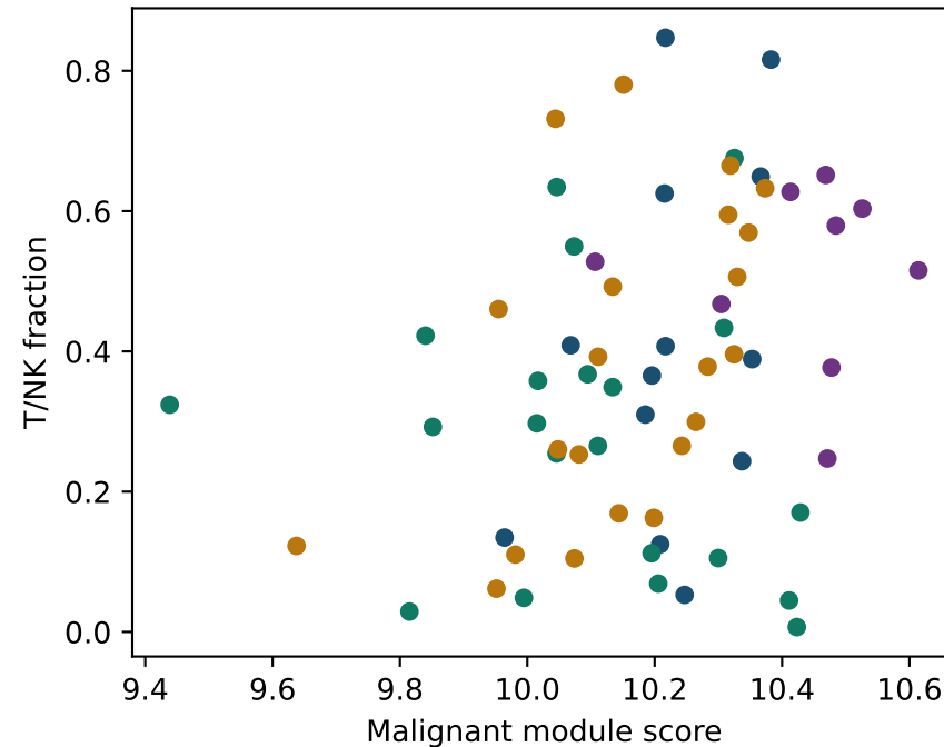
CLDN4neg ME3 (TJ-best-overlap-not-significant) DL \rho=0.214 , p=0.286 , n=65
