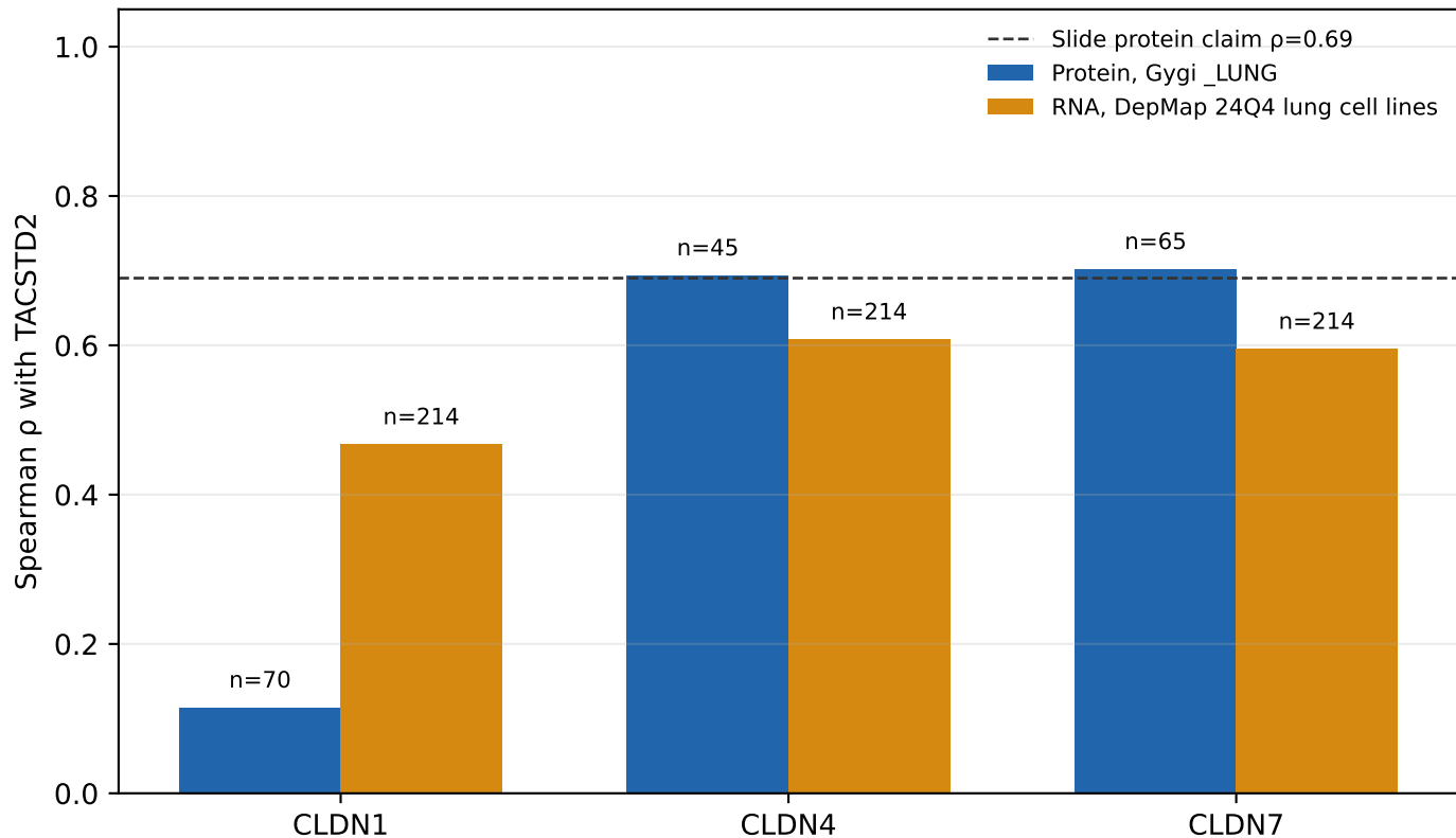
Lung-line coexpression vs the CCLE protein slide ( \rho=0.69 , n=118 )
