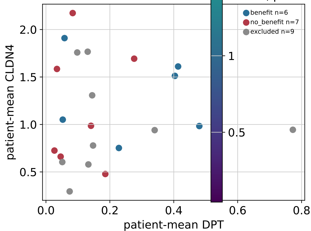
GSE205335 CLDN4 vs DPT n=22 rho=0.069, p=0.759
