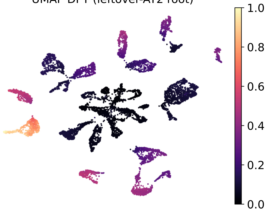
UMAP DPT (leftover-AT2 root)
