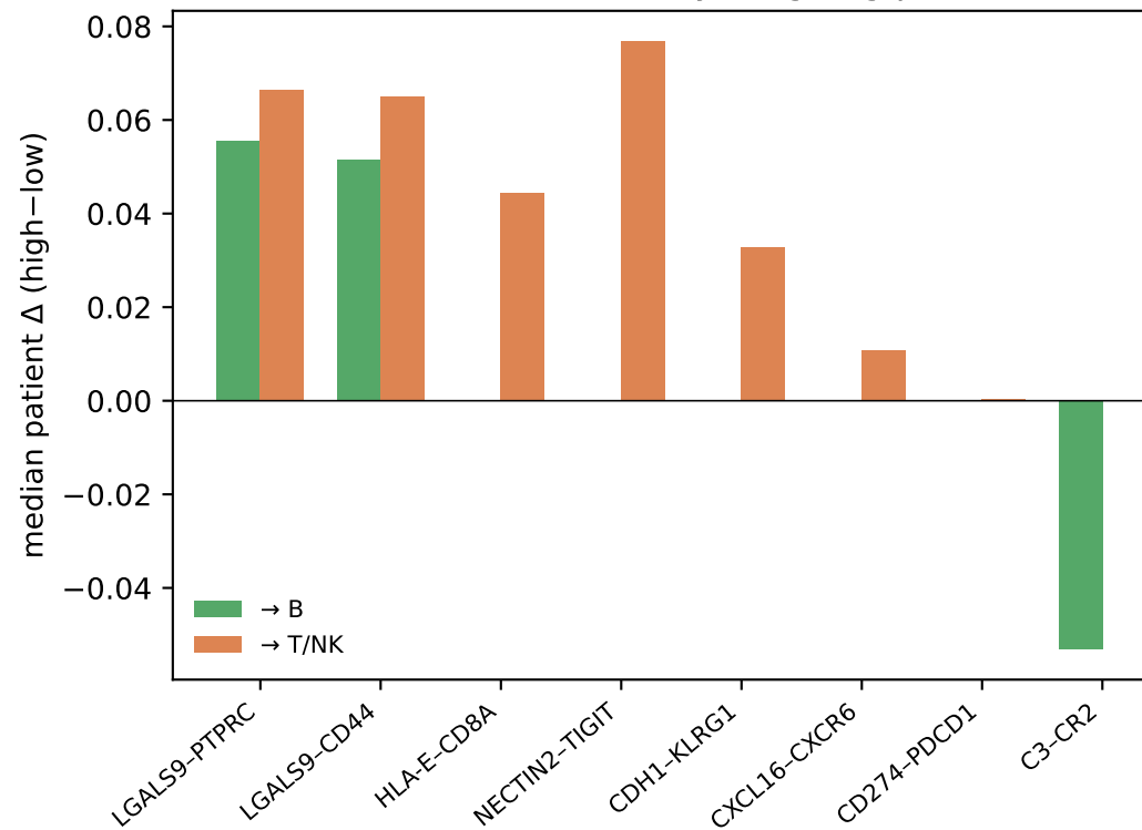
CellChat median: key outgoing pairs
