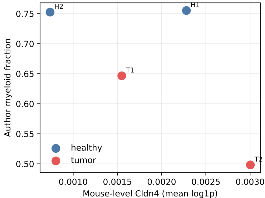
n=4 mice (2 tumor / 2 healthy) myeloid vs Cldn4
