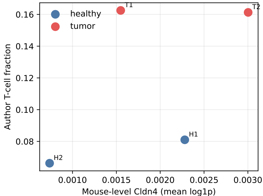
n=4 mice (2 tumor / 2 healthy) T-cell vs Cldn4
