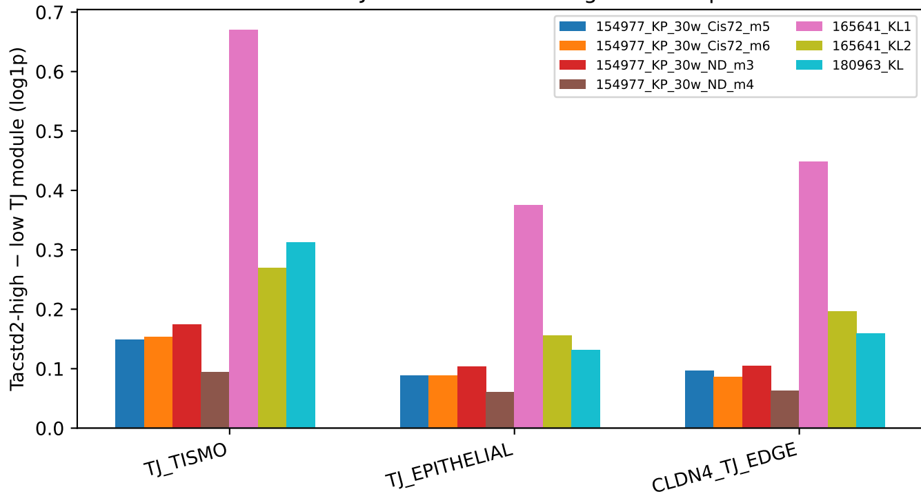
Within-mouse TJ module: Tacstd2-high vs low epithelium
