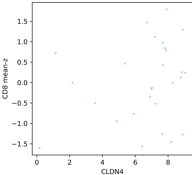
GSE135222 CLDN4 vs CD8 \rho=0.26 p=0.19 n=27
