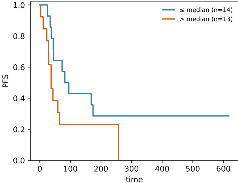
GSE135222 TJ_7gene median split PFS log-rank p=0.112
