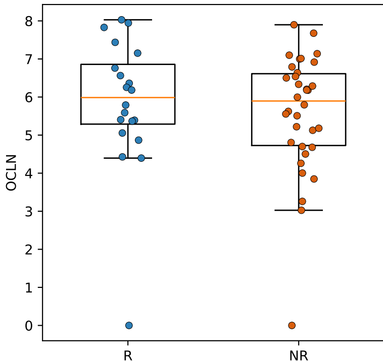
GSE161537 OCLN vs ORR (GEO RECIST CR)
