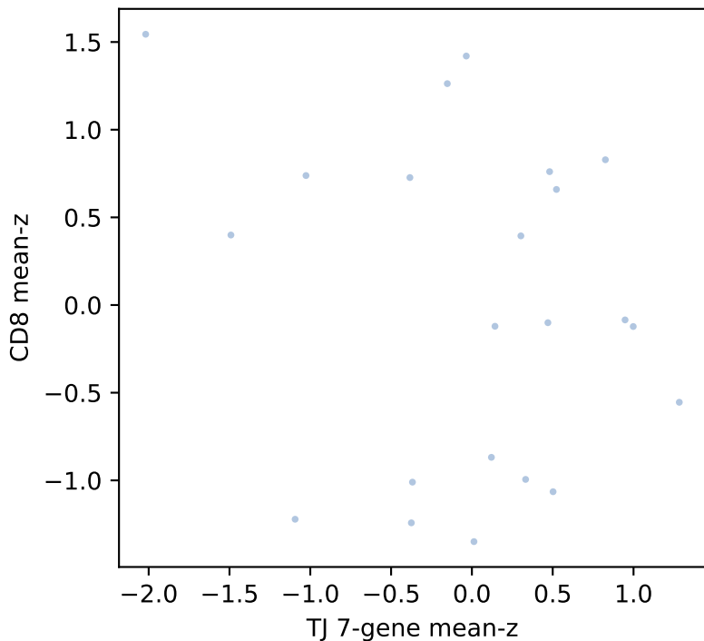
GSE166449 TJ 7-gene vs CD8 \rho=-0.10 p=0.65 n=22
