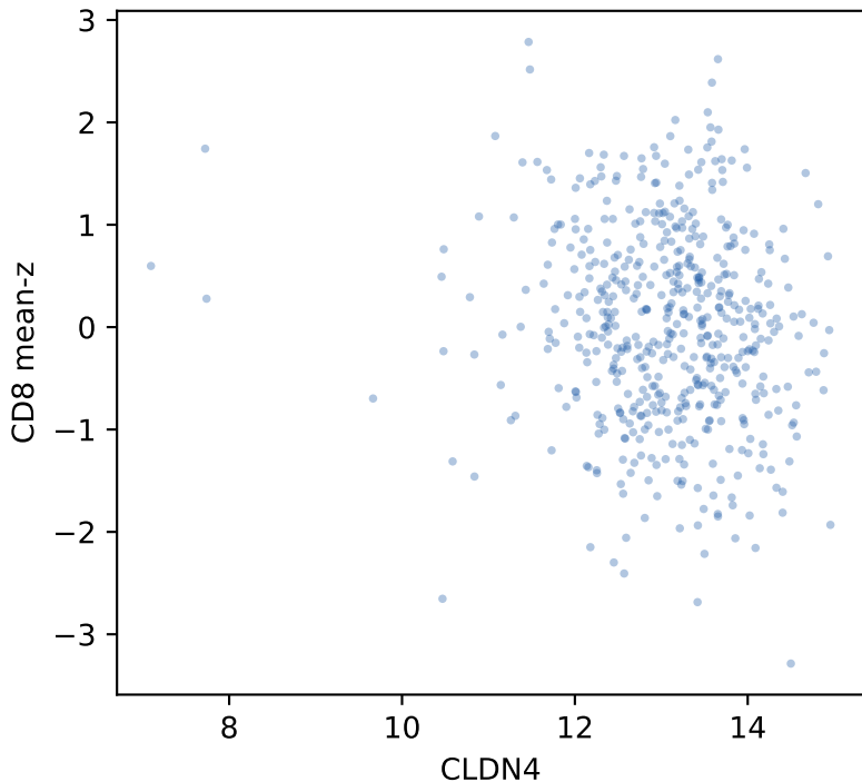
TCGA-LUAD CLDN4 vs CD8 \rho=-0.12 p=0.0087 n=515
