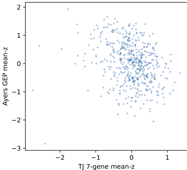
TCGA-LUAD TJ 7-gene vs GEP \rho=-0.30 p=2e-12 n=515
