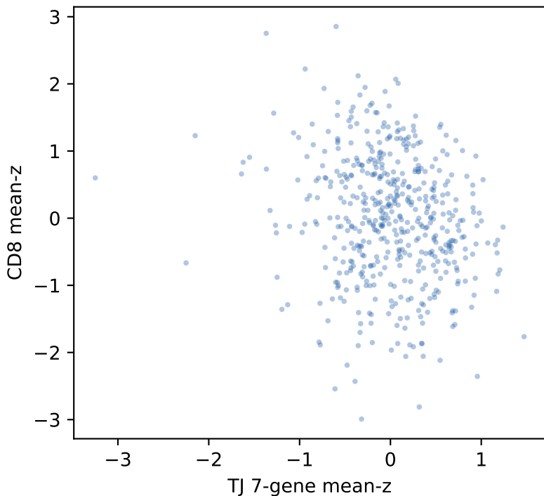
TCGA-LUSC TJ 7-gene vs CD8 \rho=-0.18 p=4.9e-05 n=502
