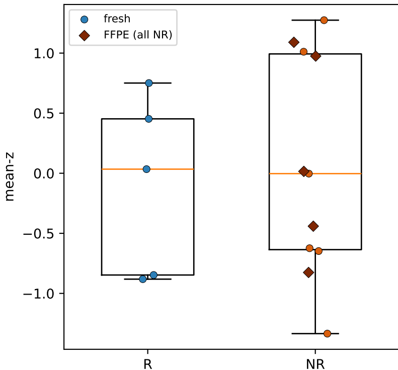
GSE126044 basal/squamous keratin mean-z
