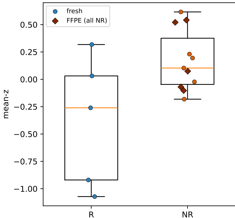
GSE126044 Reactome TJ mean-z
