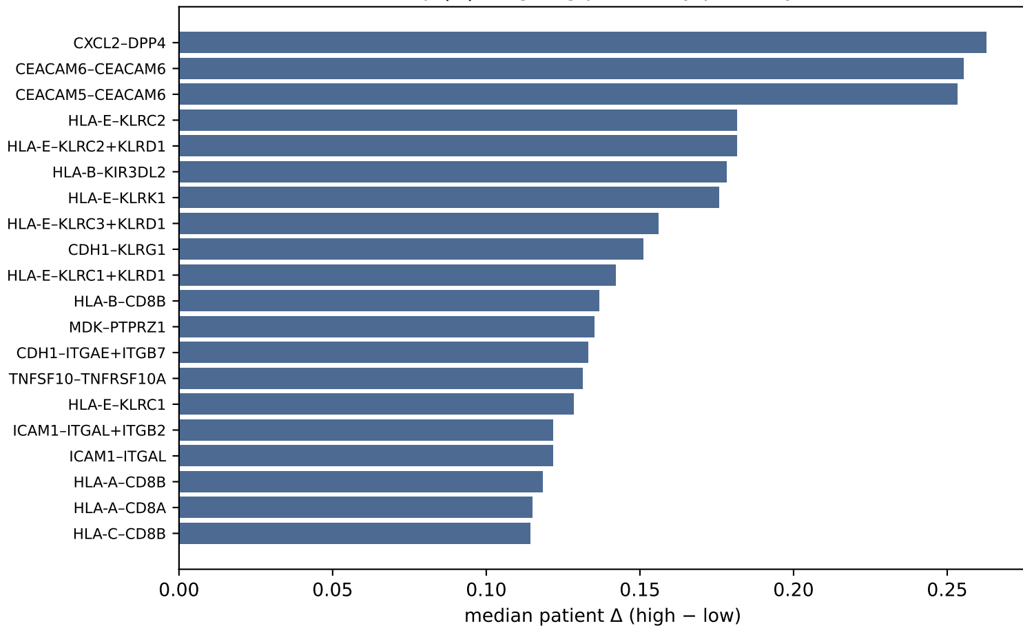
Top |\Delta| outgoing pairs (any pathway)
