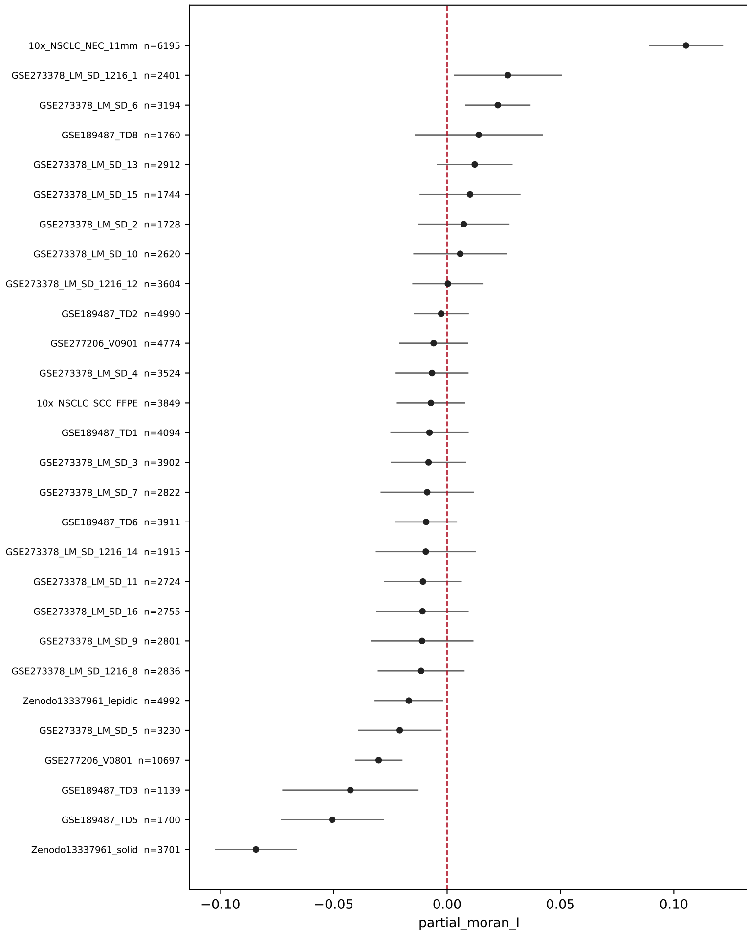
Partial bivariate Moran's I (KRT8 residuals)
