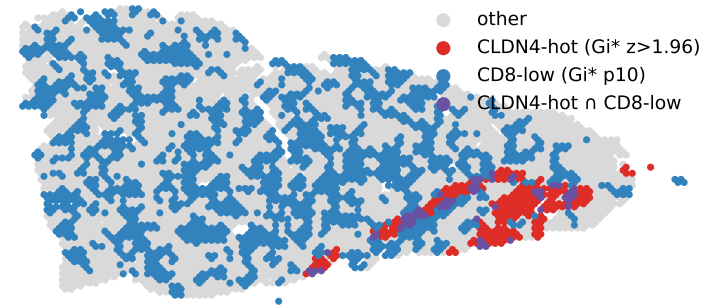
Gi* overlay I=+0.103 hotnCD8-low=61/6195
