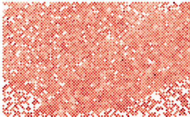
GSE189487_TD2 CLDN4 (log CP10k)
