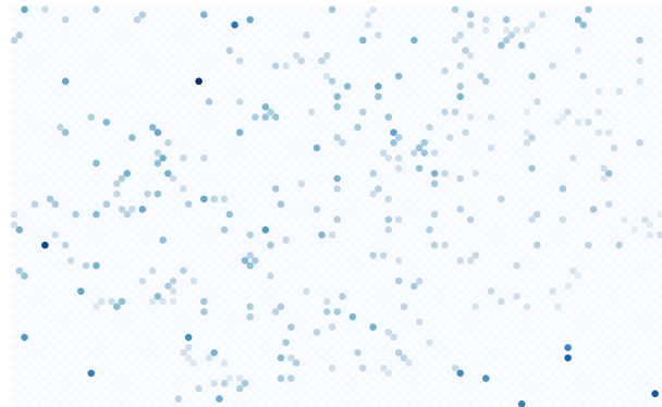
CD8A (log CP10k)
