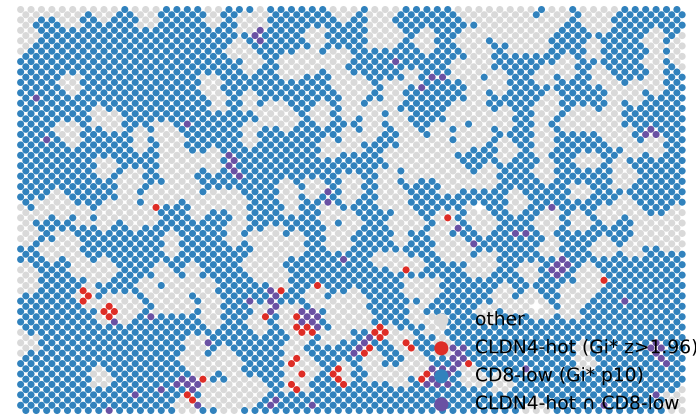
Gi* overlay I=-0.002 hotnCD8-low=91/4990
