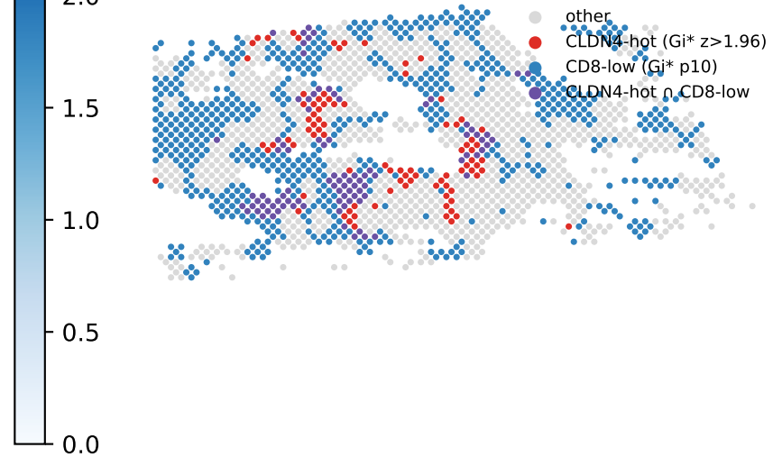
Gi* overlay I=-0.053 hotnCD8-low=92/1728
