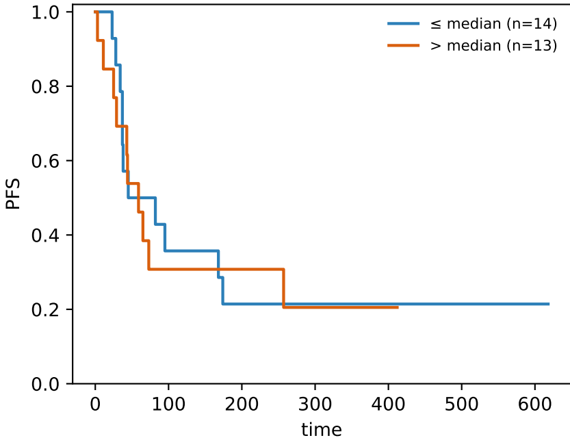
GSE135222 CLDN4 median split PFS log-rank p=0.909
