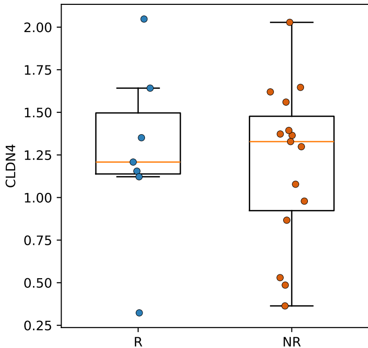
SE166449 CLDN4 vs GEO immunotherapy responder vs non-
