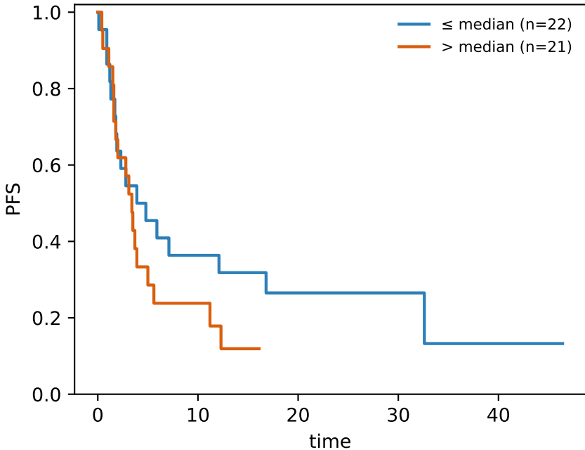
GSE190265 TJ_7gene median split PFS log-rank p=0.242
