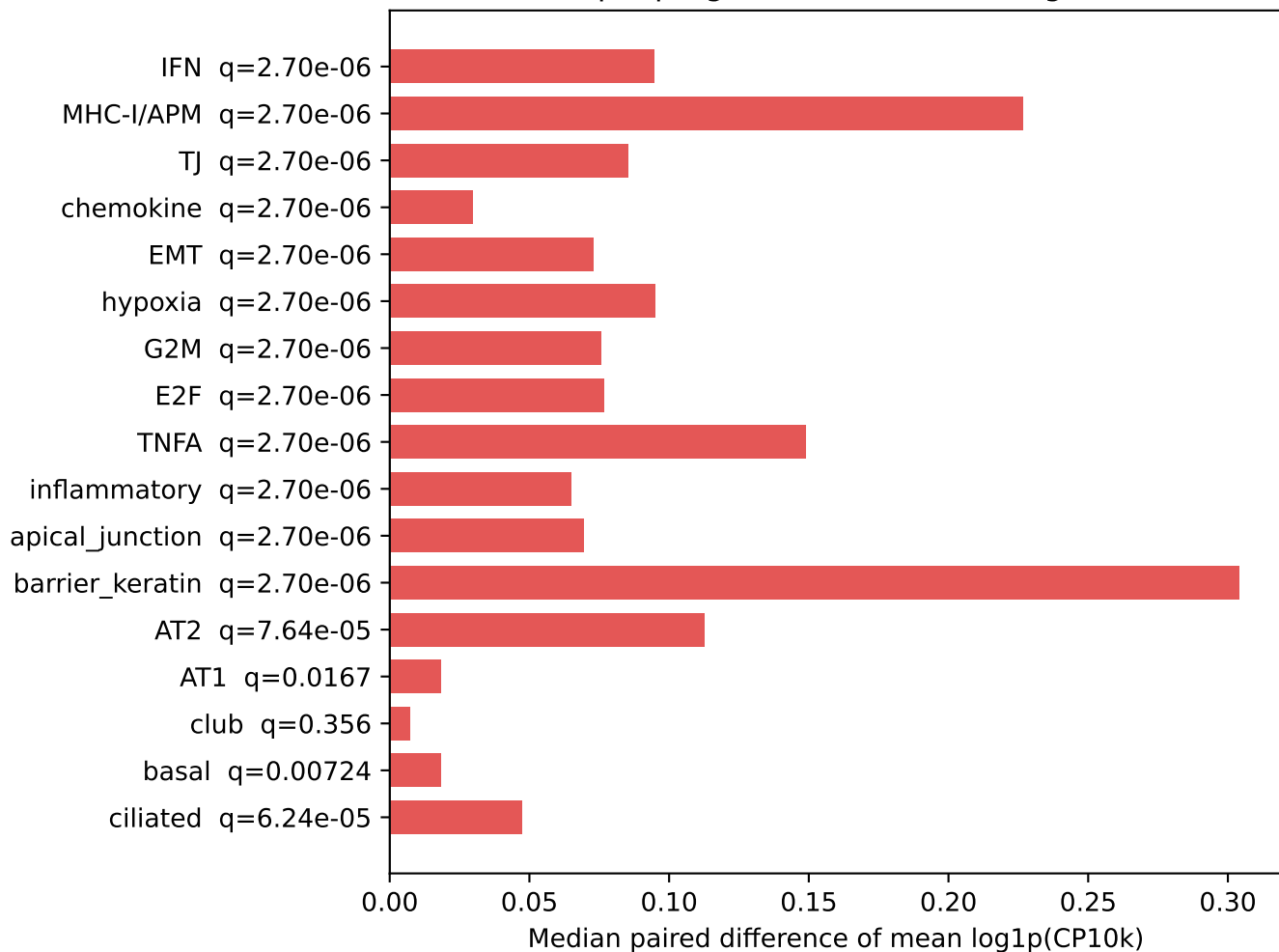
Within-sample program score, CLDN4-high minus low
