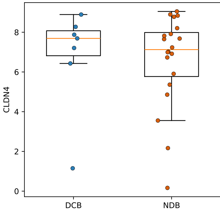
GSE135222 CLDN4 vs DCB (PFS \geq 183d)
